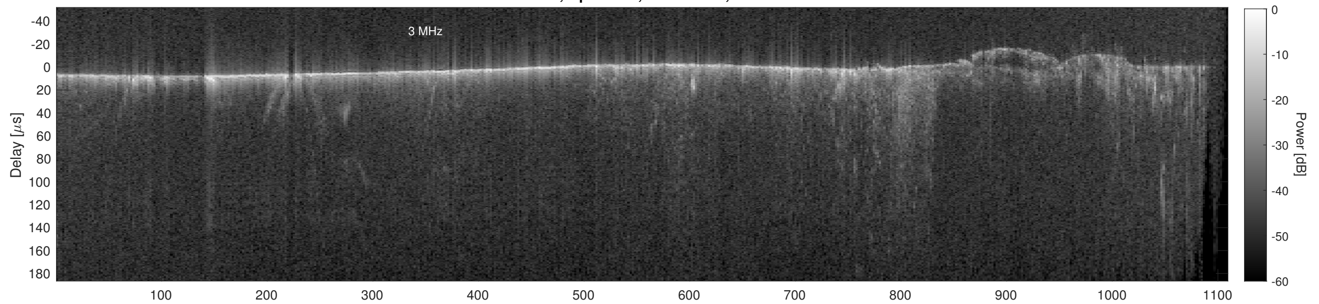
Orbit 12058, Cluttergram
