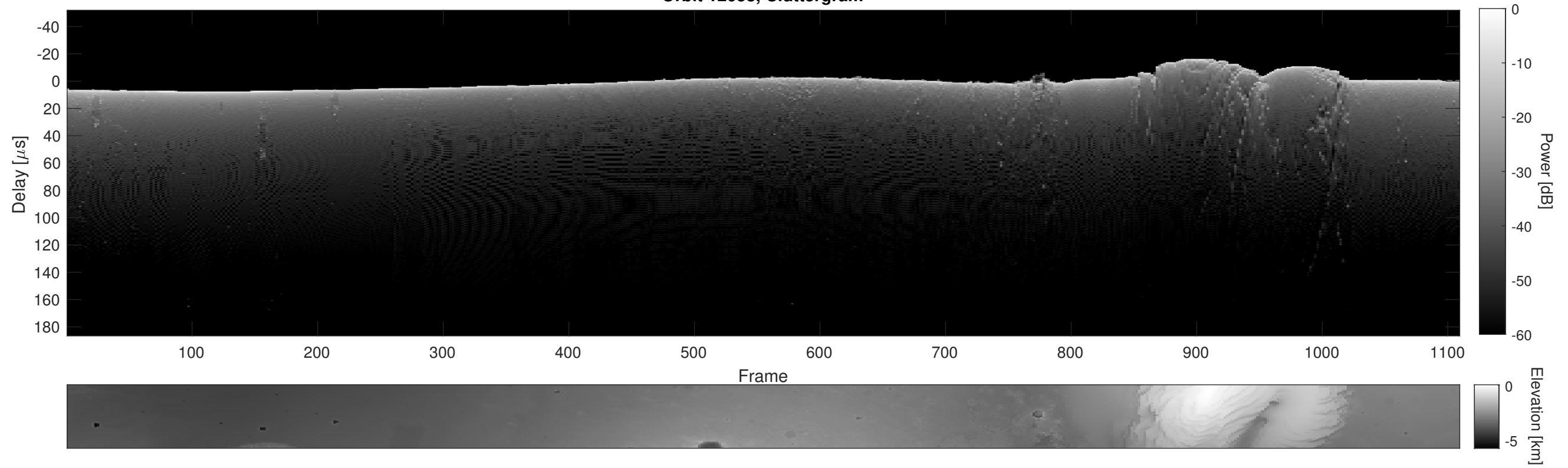
Orbit 12058, Cluttergram
