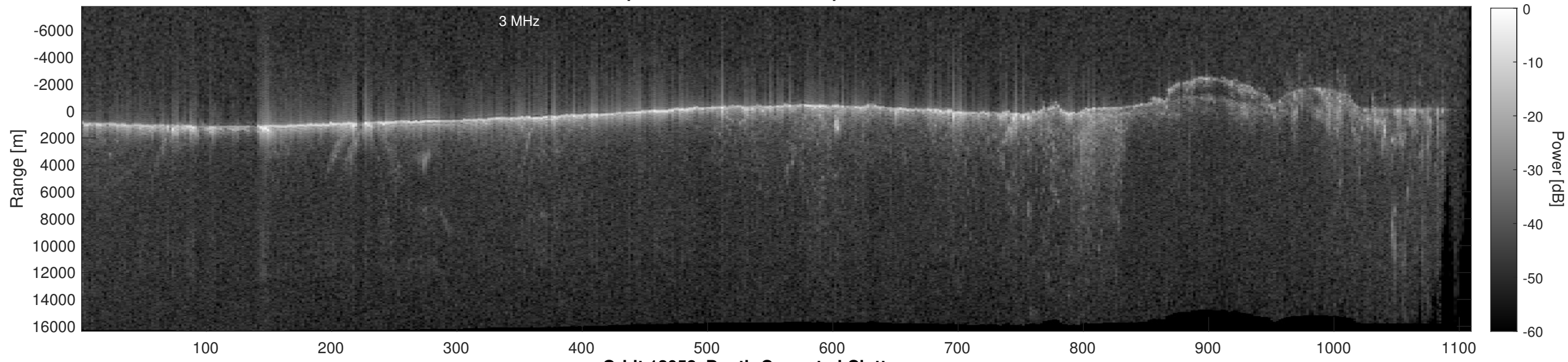
Orbit 12058, Depth-Corrected Cluttergram
