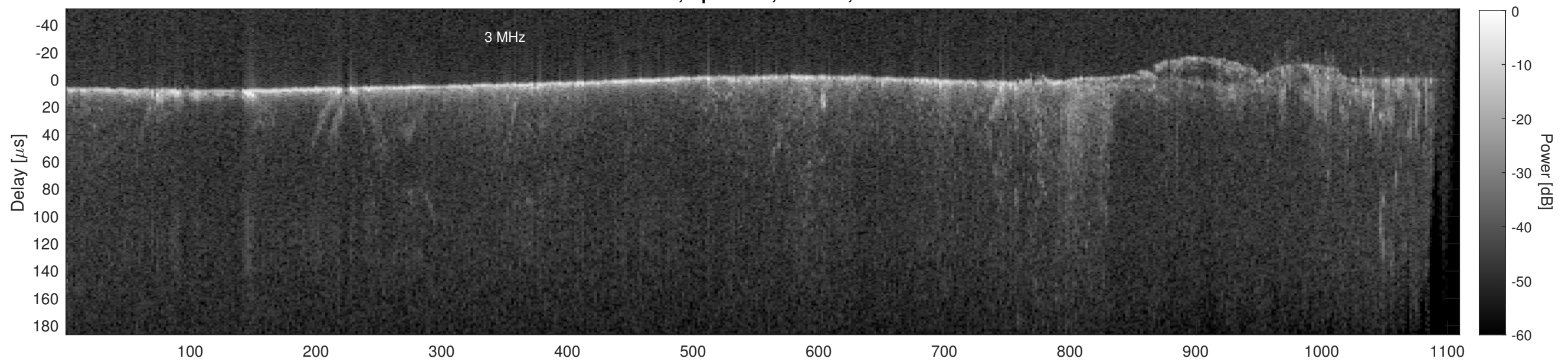
Orbit 12058, Cluttergram
