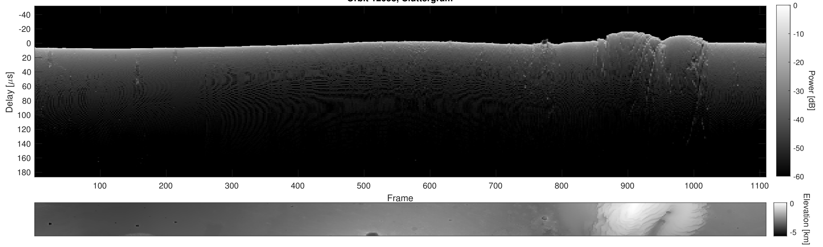
Orbit 12058, Cluttergram
