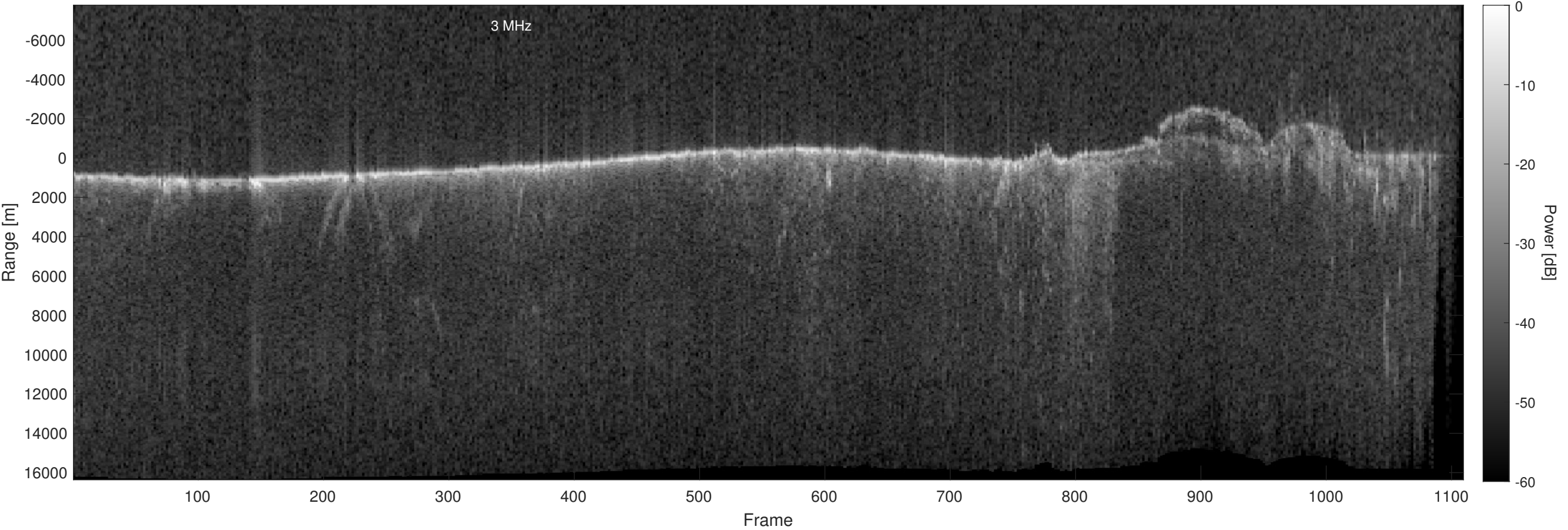
Orbit 12058, Optimized, Window, Depth-Corrected, Channel 2
