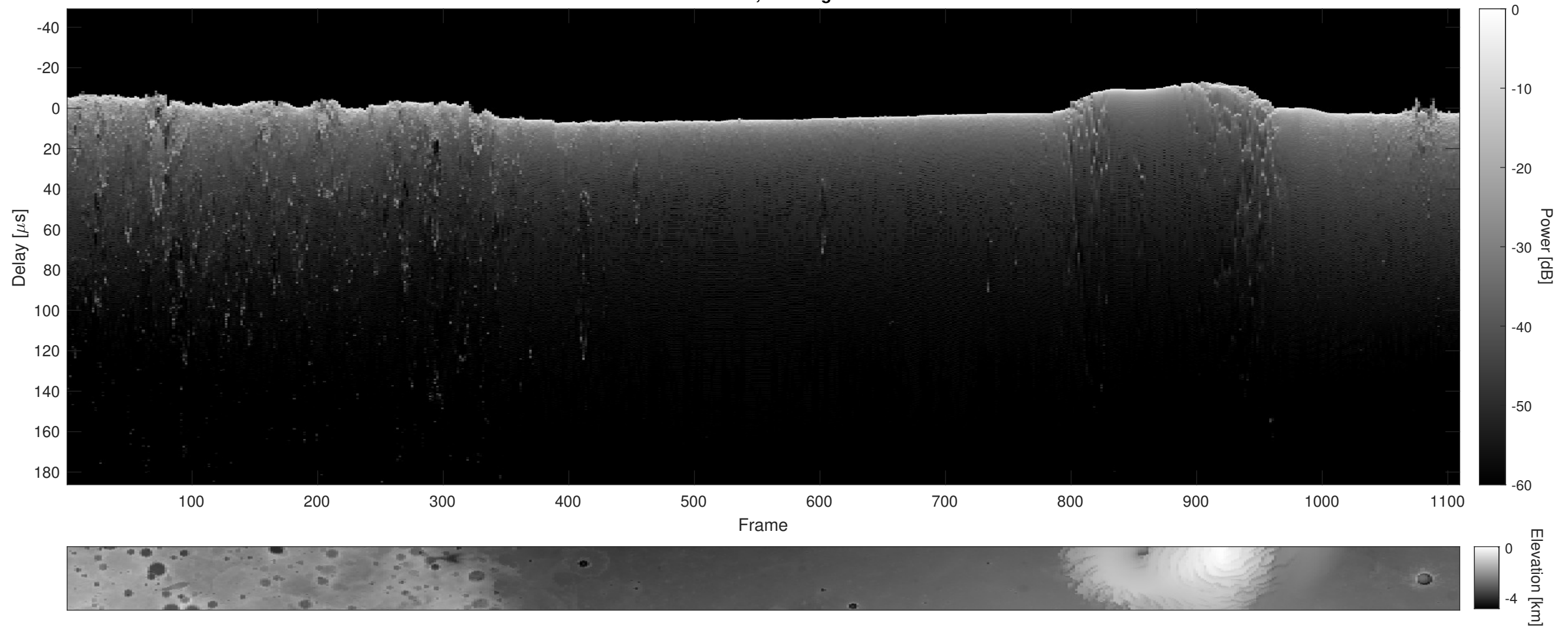
Orbit 12060, Cluttergram
