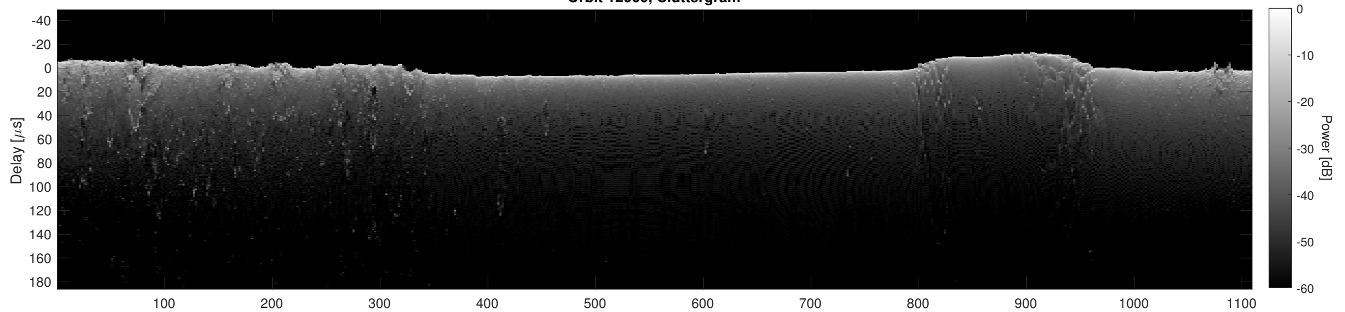
Orbit 12060, Cluttergram
