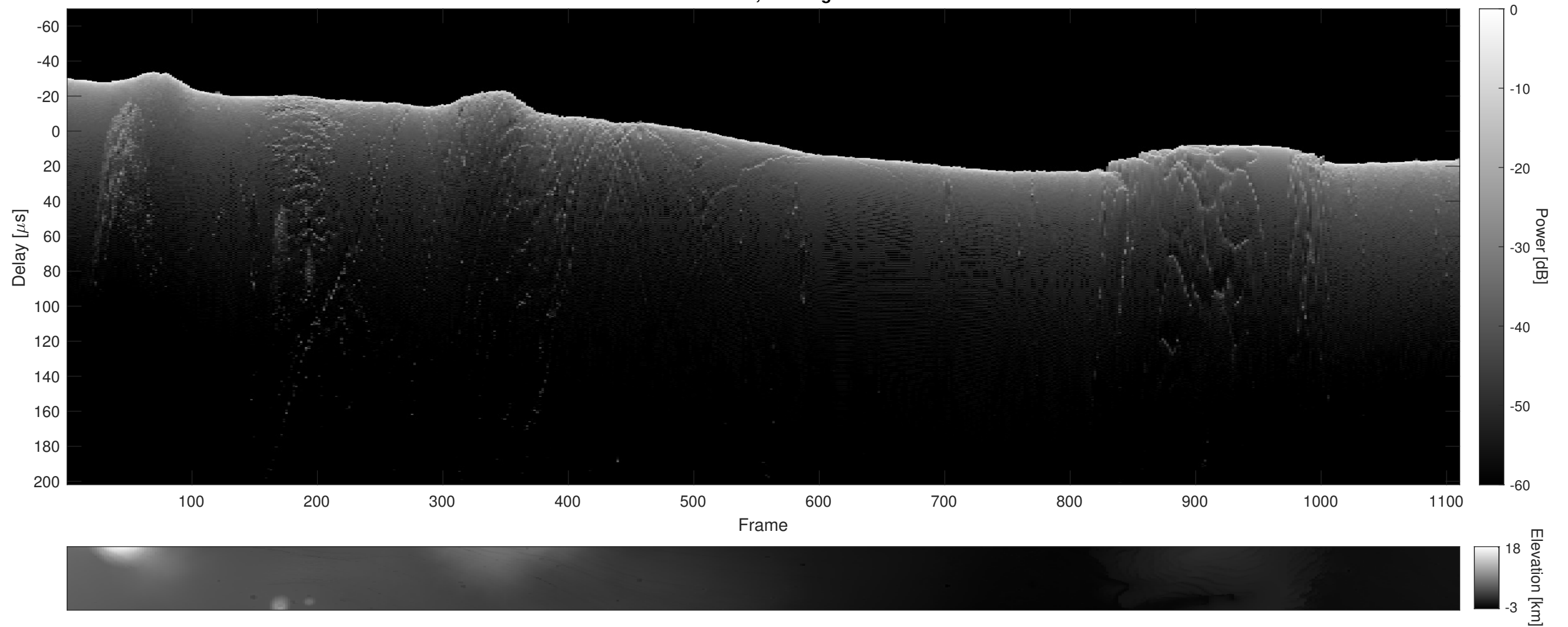
Orbit 12061, Cluttergram
