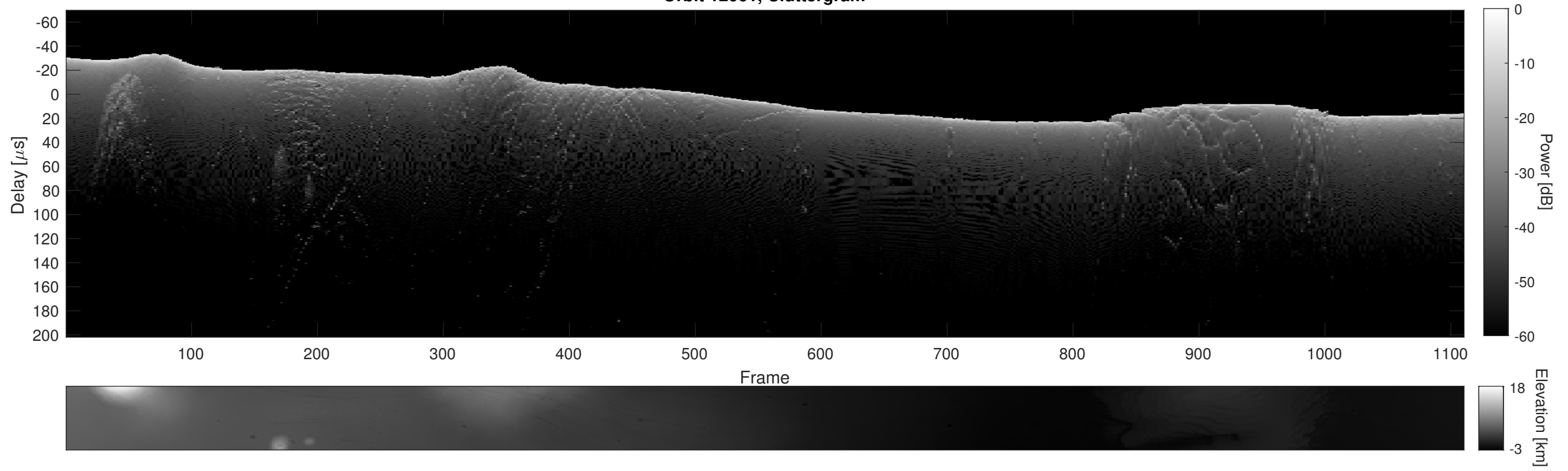
Orbit 12061, Cluttergram
