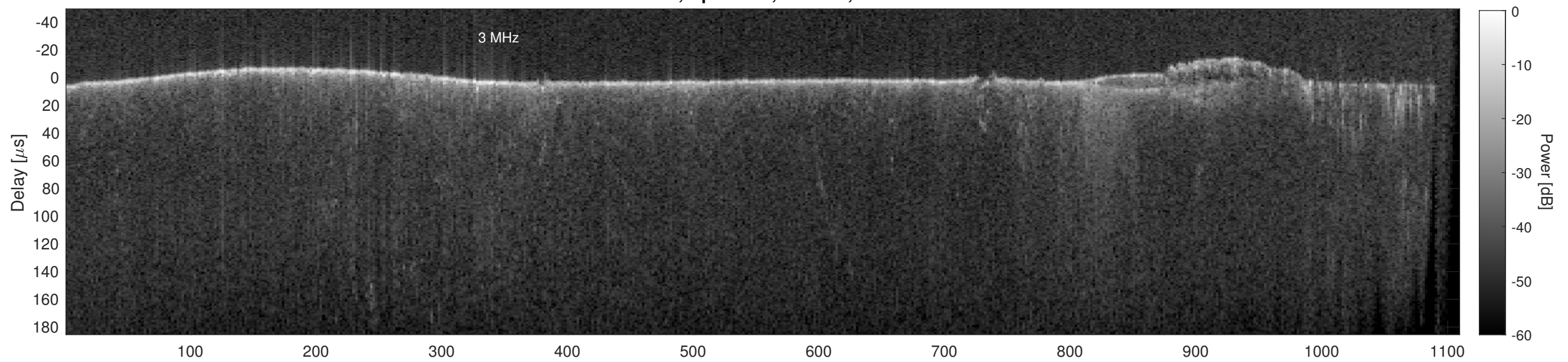
Orbit 12062, Cluttergram
