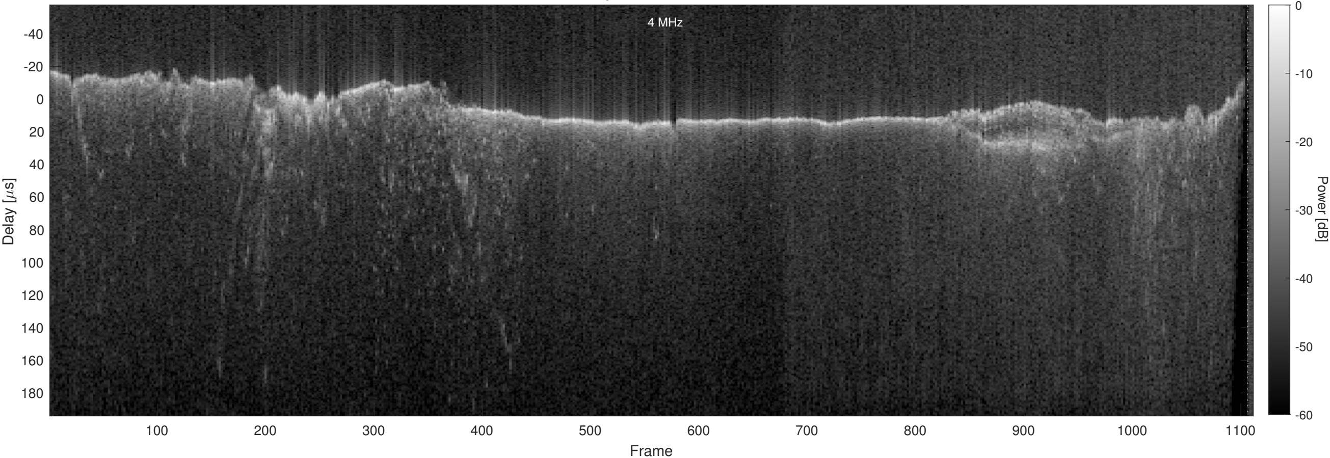
Orbit 12063, Chapman, No Window, Channel 2
