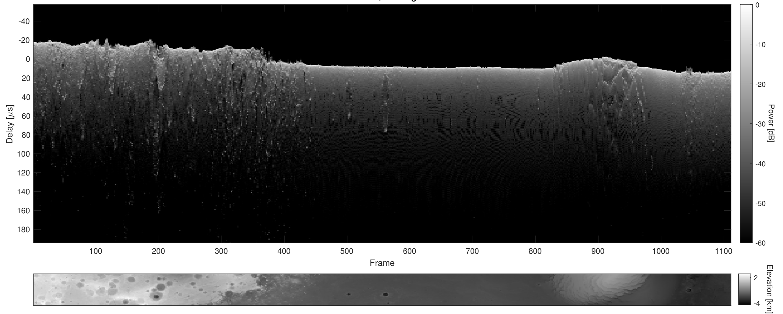
Orbit 12063, Cluttergram
