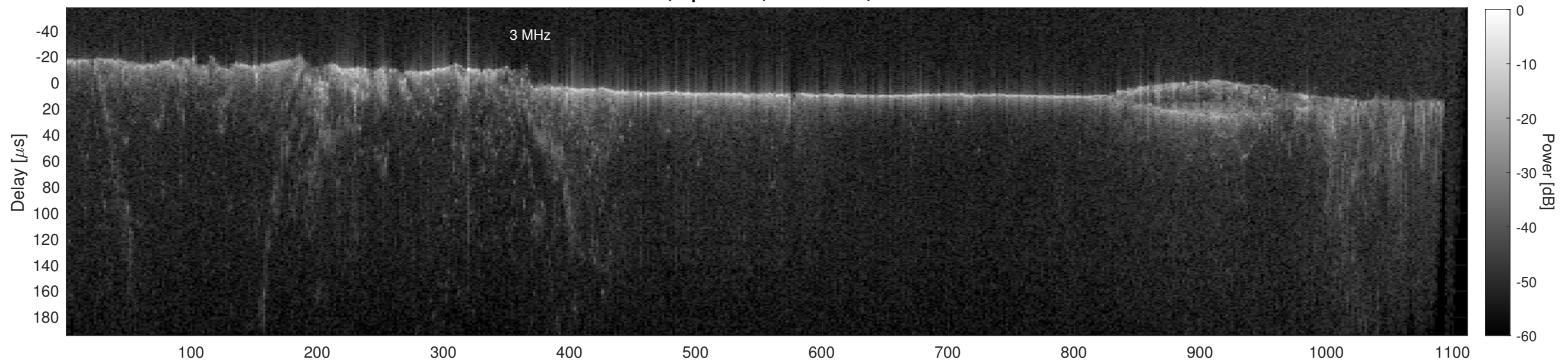
Orbit 12063, Cluttergram
