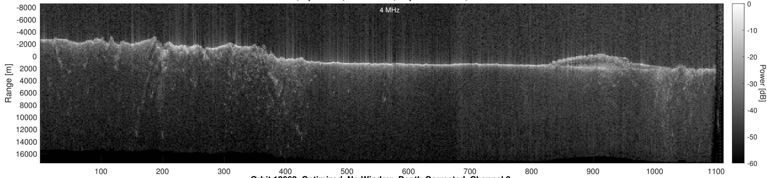
Orbit 12063, Optimized, No Window, Depth-Corrected, Channel 2
