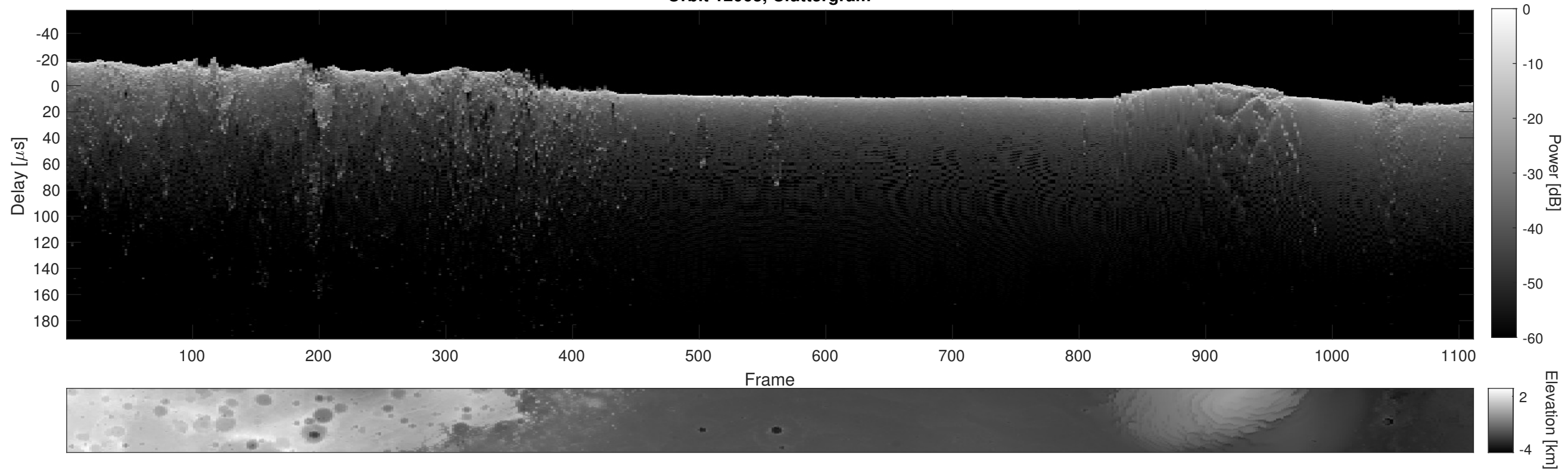
Orbit 12063, Cluttergram
