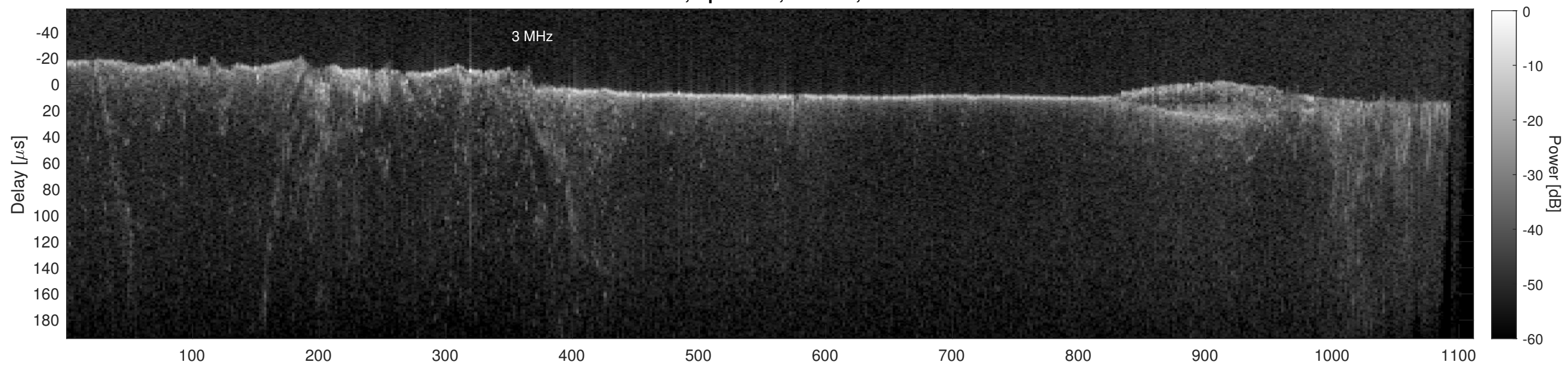
Orbit 12063, Cluttergram
