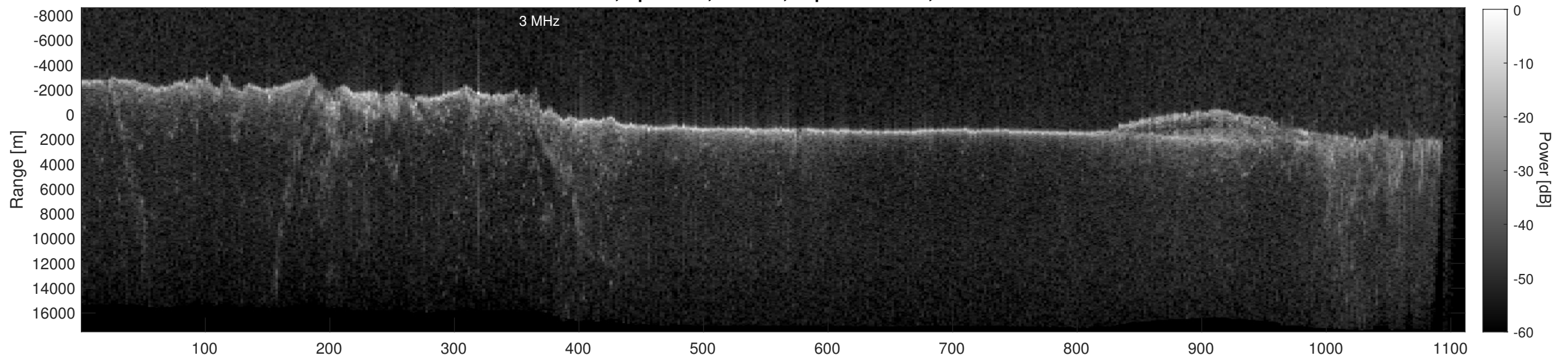
Orbit 12063, Depth-Corrected Cluttergram
