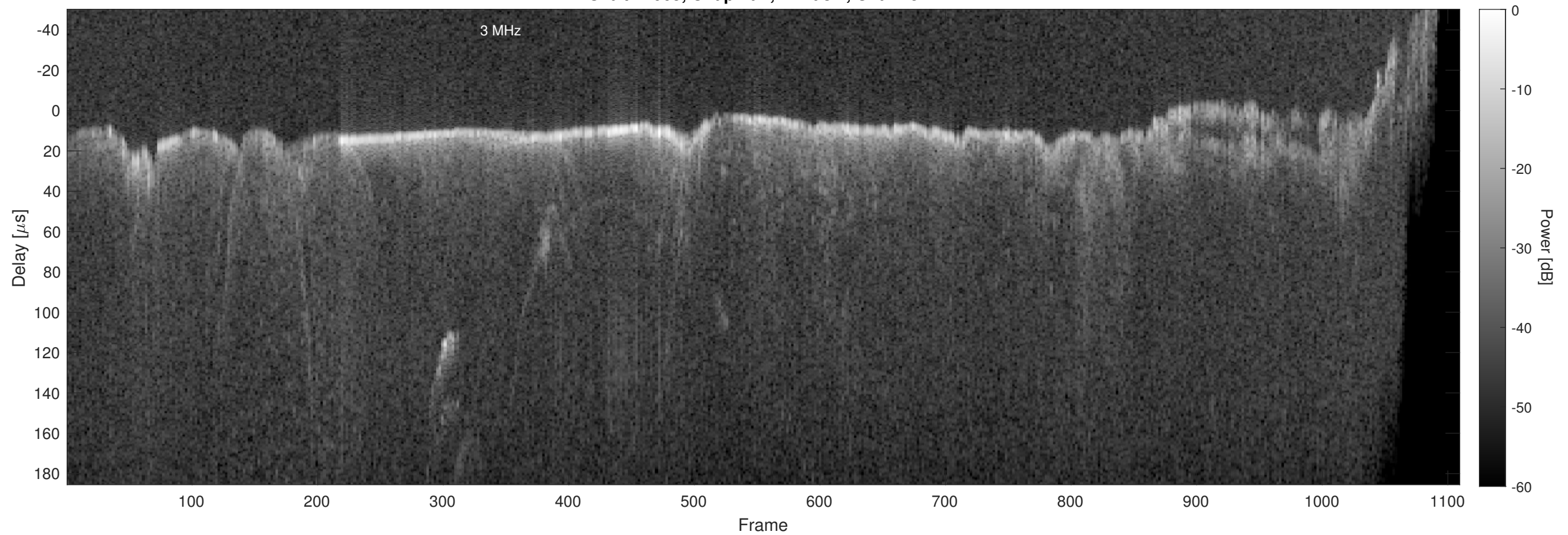
Orbit 12065, Chapman, Window, Channel 2
