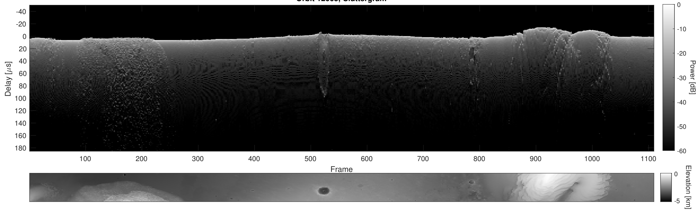
Orbit 12065, Cluttergram
