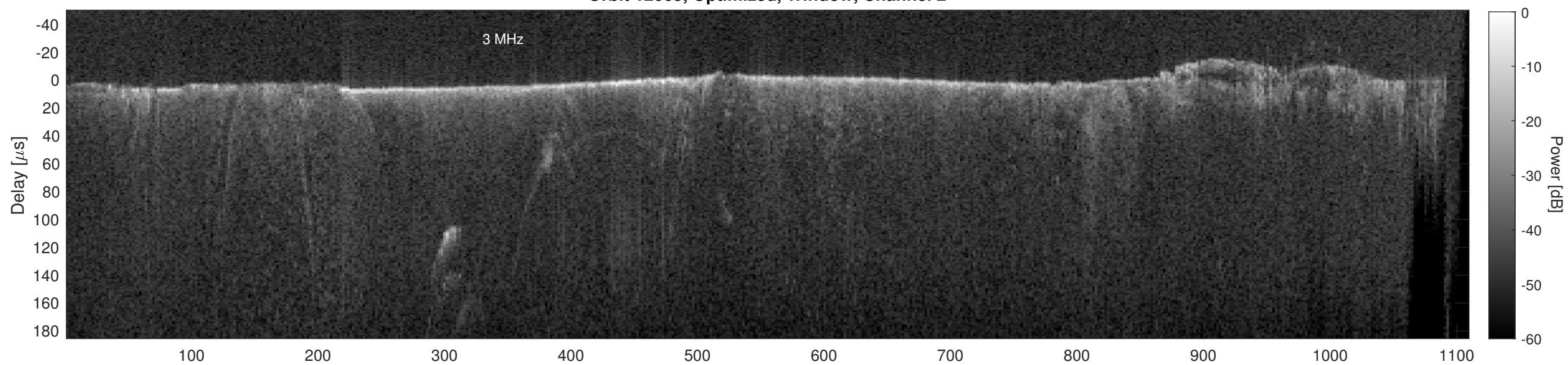
Orbit 12065, Cluttergram
