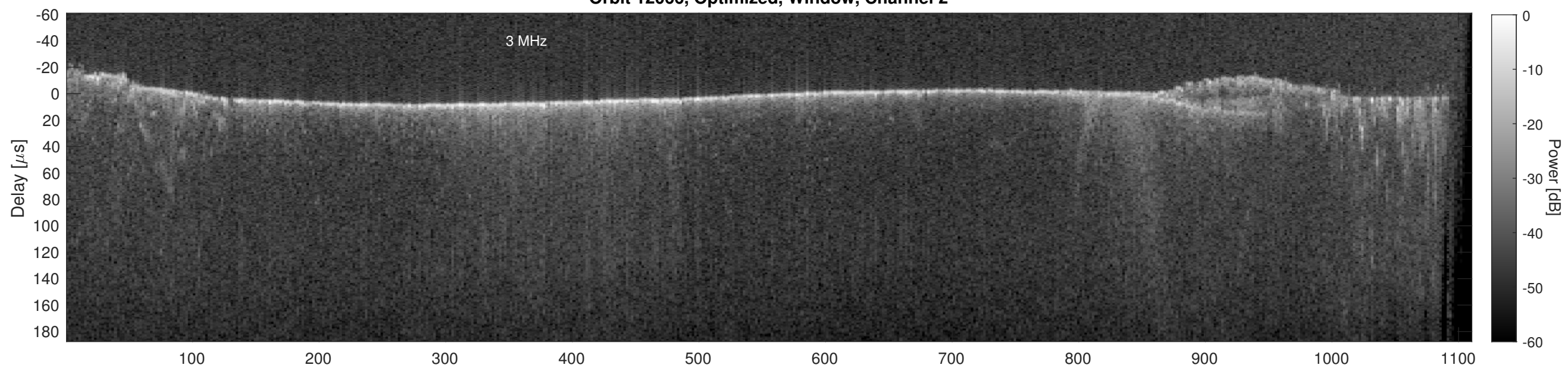
Orbit 12066, Cluttergram
