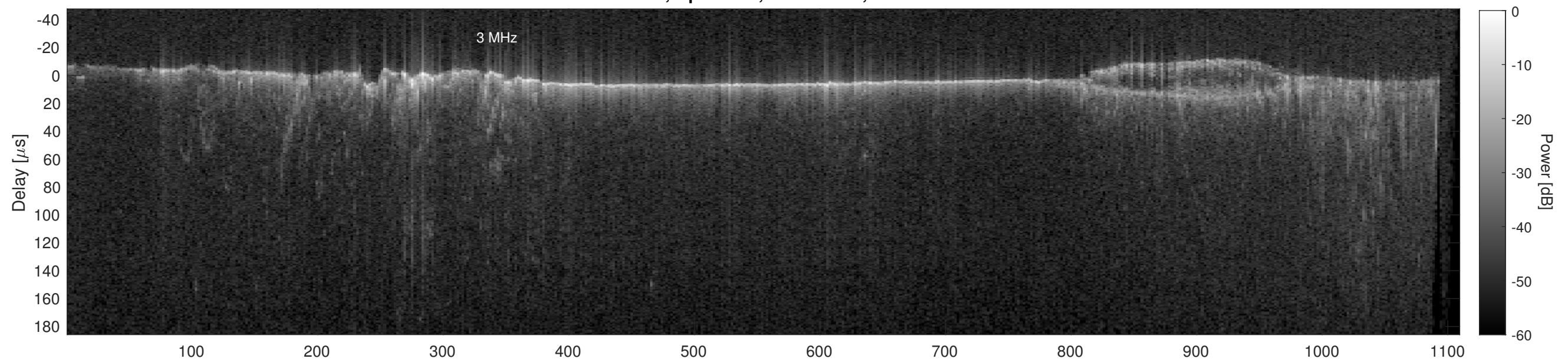
Orbit 12067, Cluttergram
