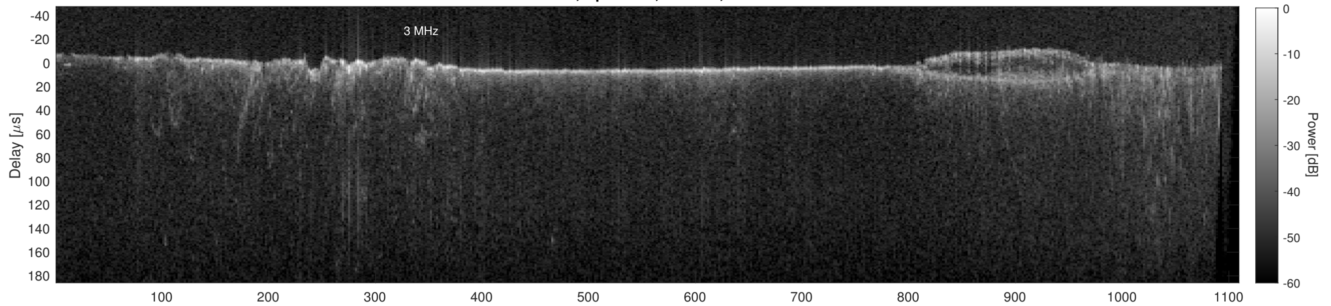
Orbit 12067, Cluttergram
