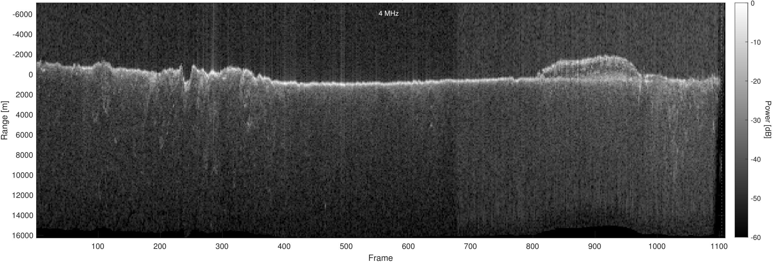
Orbit 12067, Optimized, Window, Depth-Corrected, Channel 2
