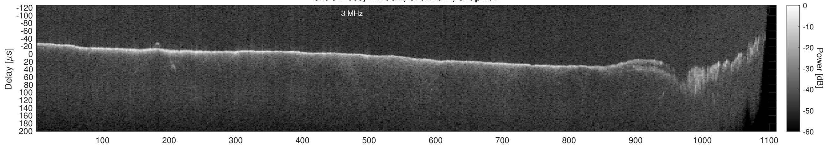
Orbit 12068, Window, Channel 2, Optimized
