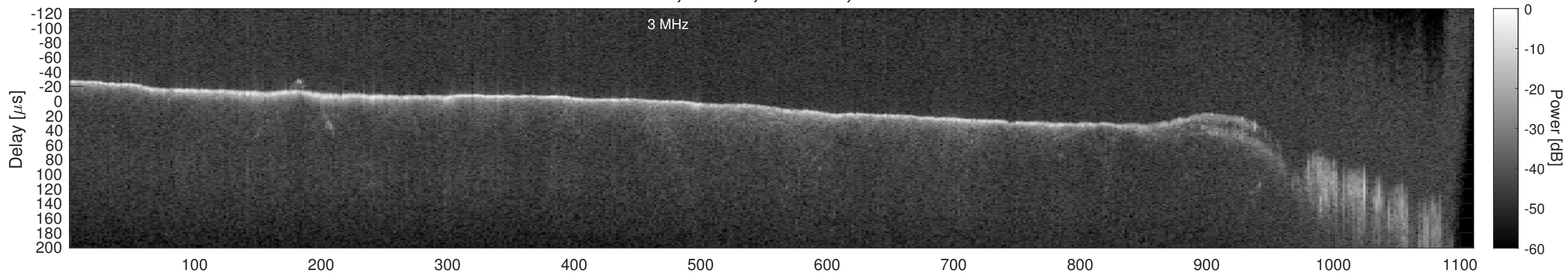
Orbit 12068, Window, Channel 2, Chapman
