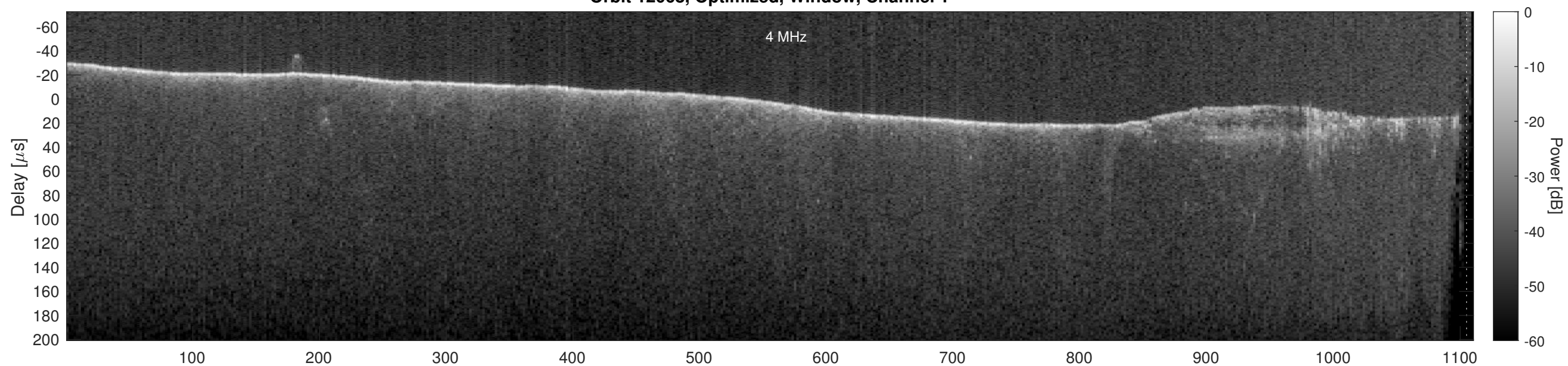
Orbit 12068, Optimized, Window, Channel 2
