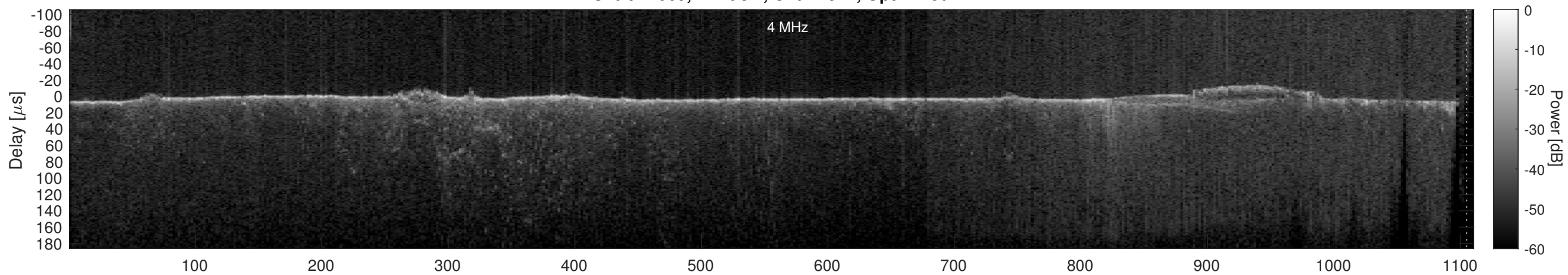
Orbit 12069, Cluttergram
