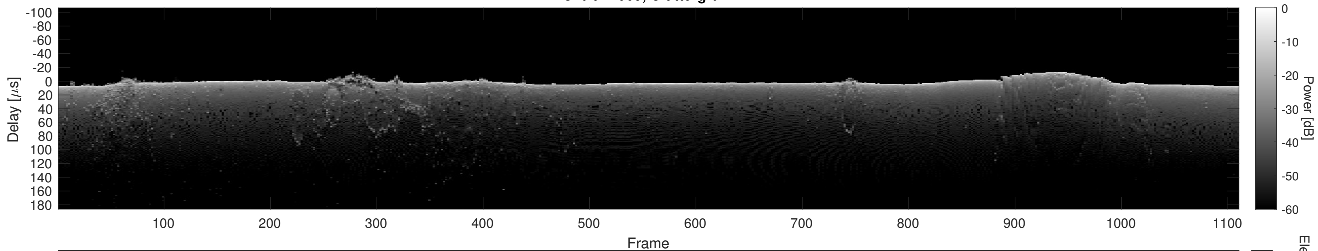
Orbit 12069, Cluttergram
