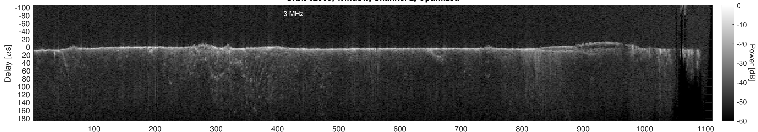
Orbit 12069, Cluttergram
