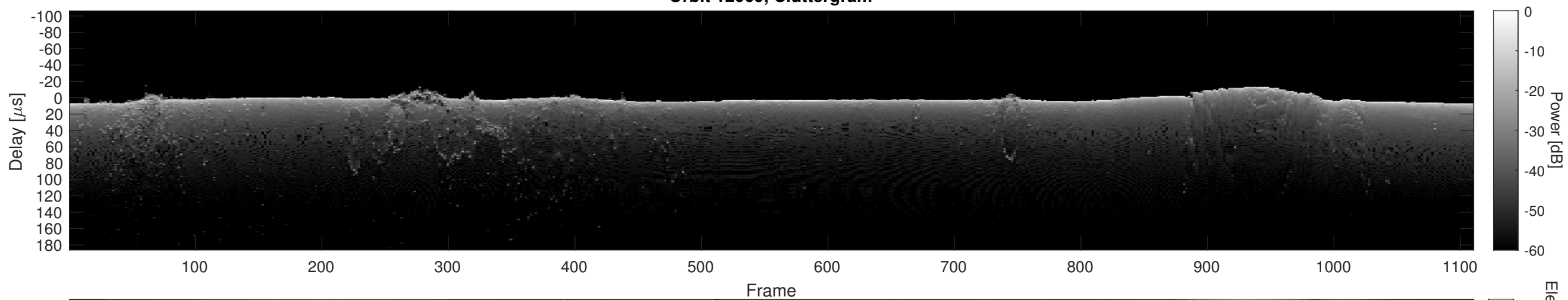
Orbit 12069, Cluttergram
