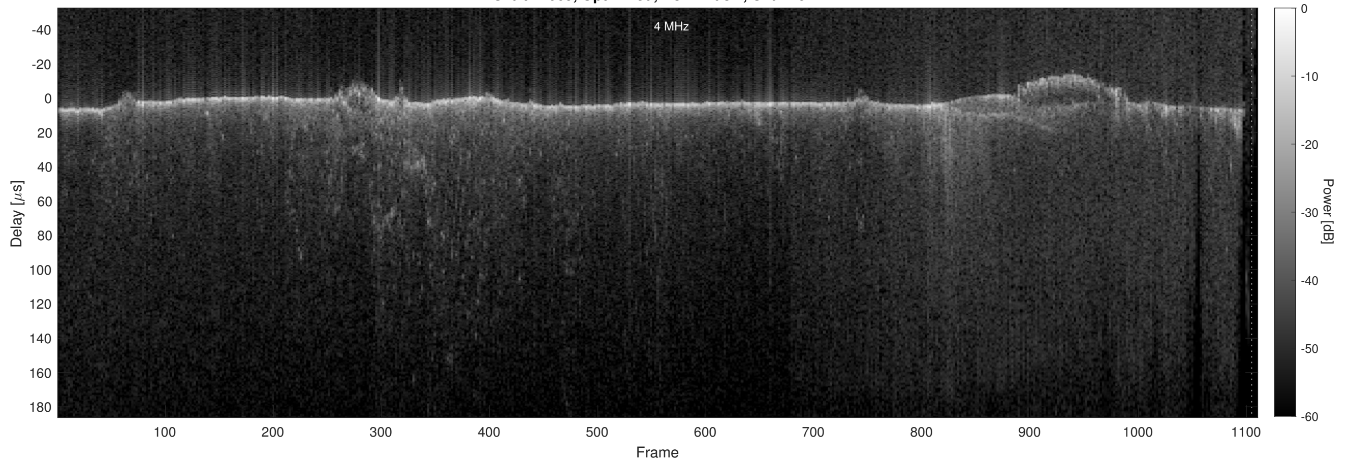
Orbit 12069, Optimized, No Window, Channel 2
