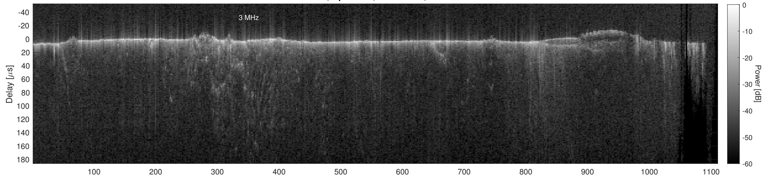
Orbit 12069, Cluttergram
