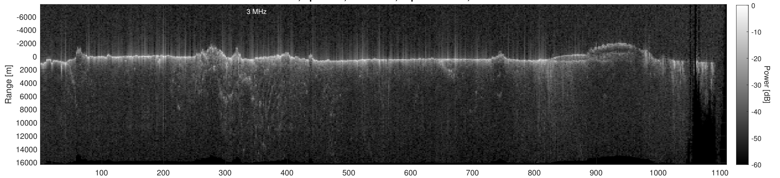
Orbit 12069, Depth-Corrected Cluttergram
