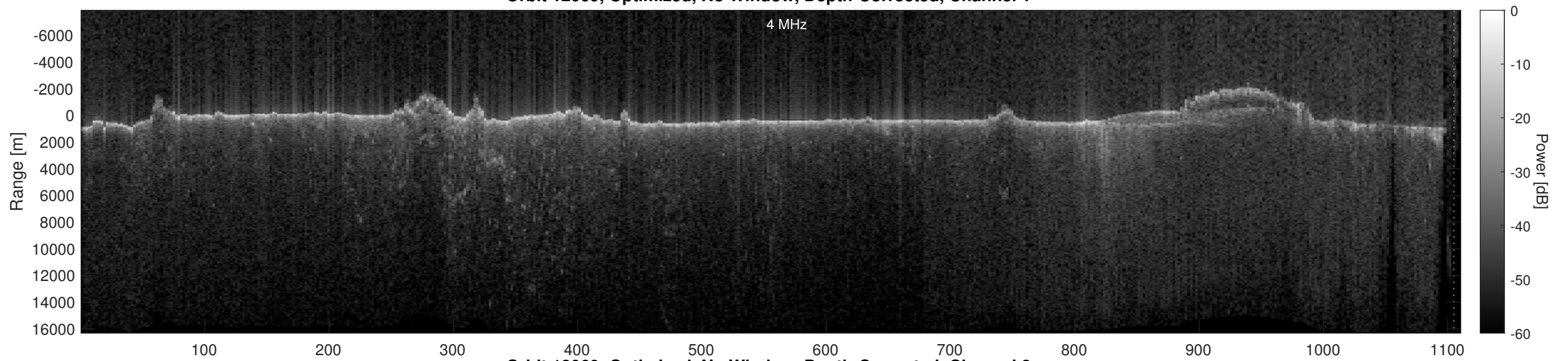
Orbit 12069, Optimized, No Window, Depth-Corrected, Channel 2
