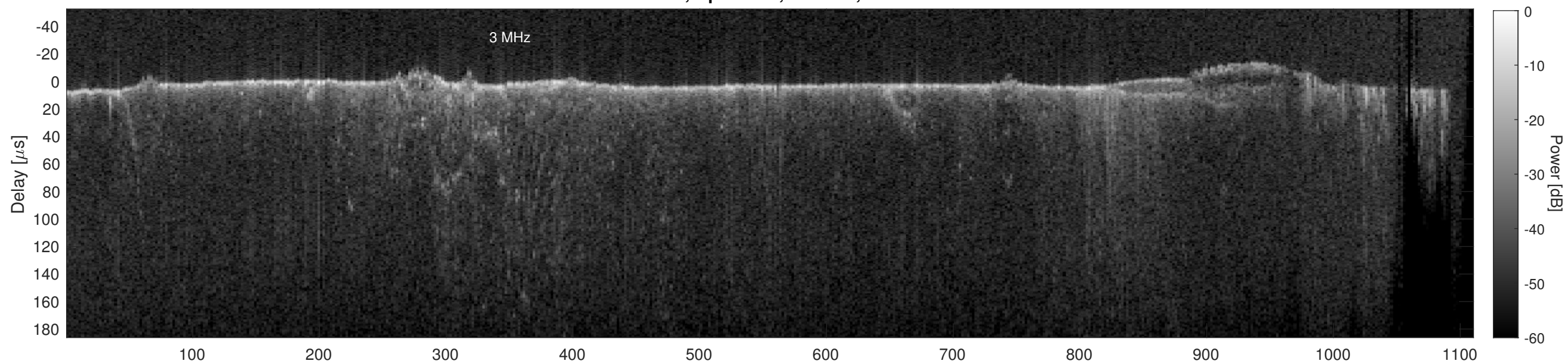
Orbit 12069, Cluttergram
