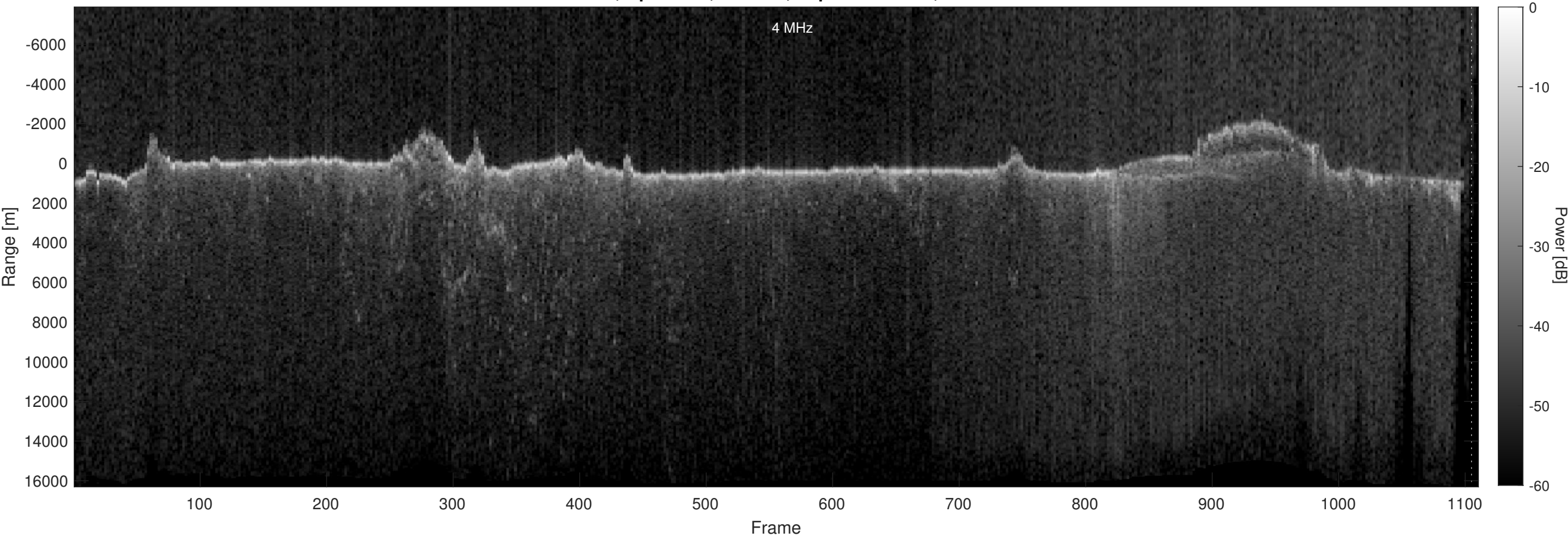
Orbit 12069, Optimized, Window, Depth-Corrected, Channel 2
