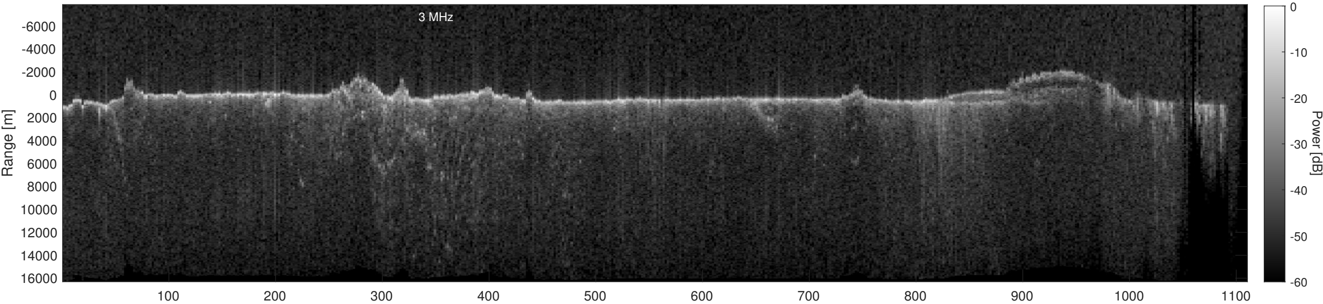
Orbit 12069, Depth-Corrected Cluttergram
