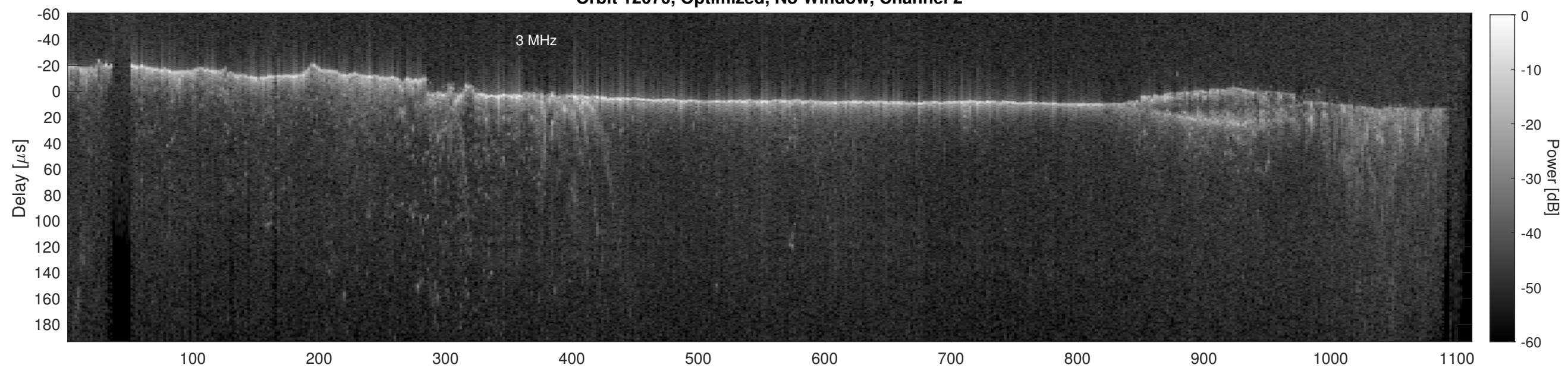
Orbit 12070, Cluttergram
