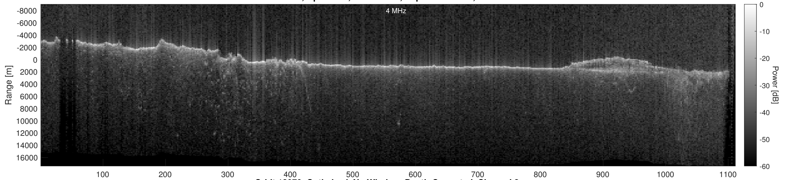
Orbit 12070, Optimized, No Window, Depth-Corrected, Channel 2
