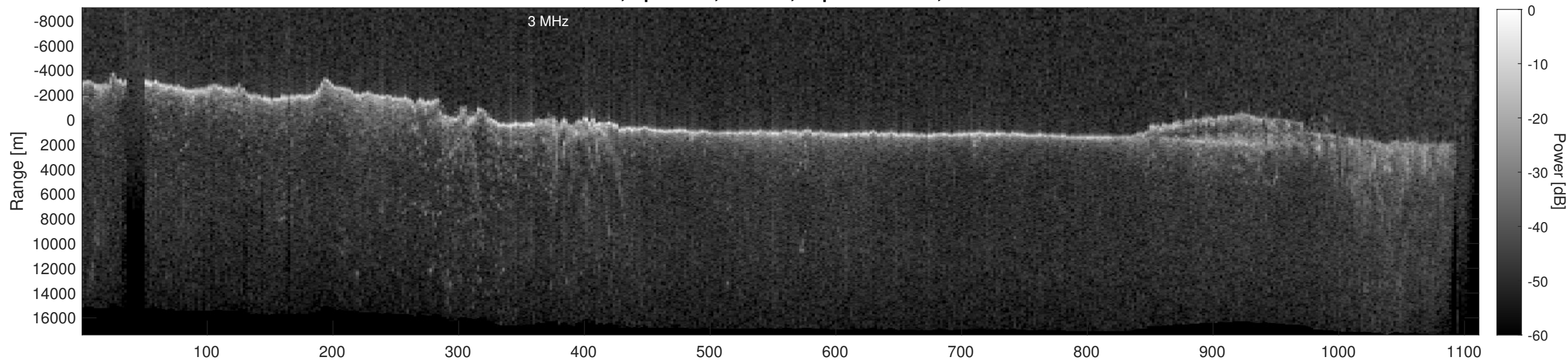
Orbit 12070, Depth-Corrected Cluttergram
