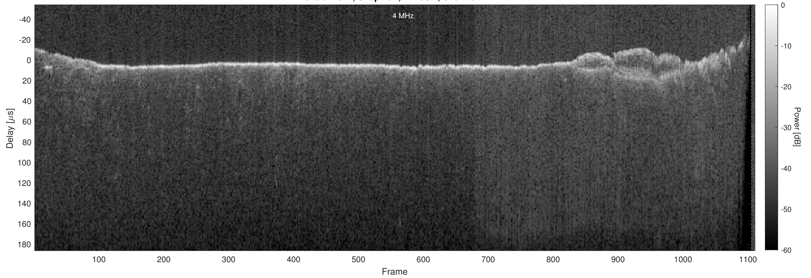
Orbit 12071, Chapman, Window, Channel 2
