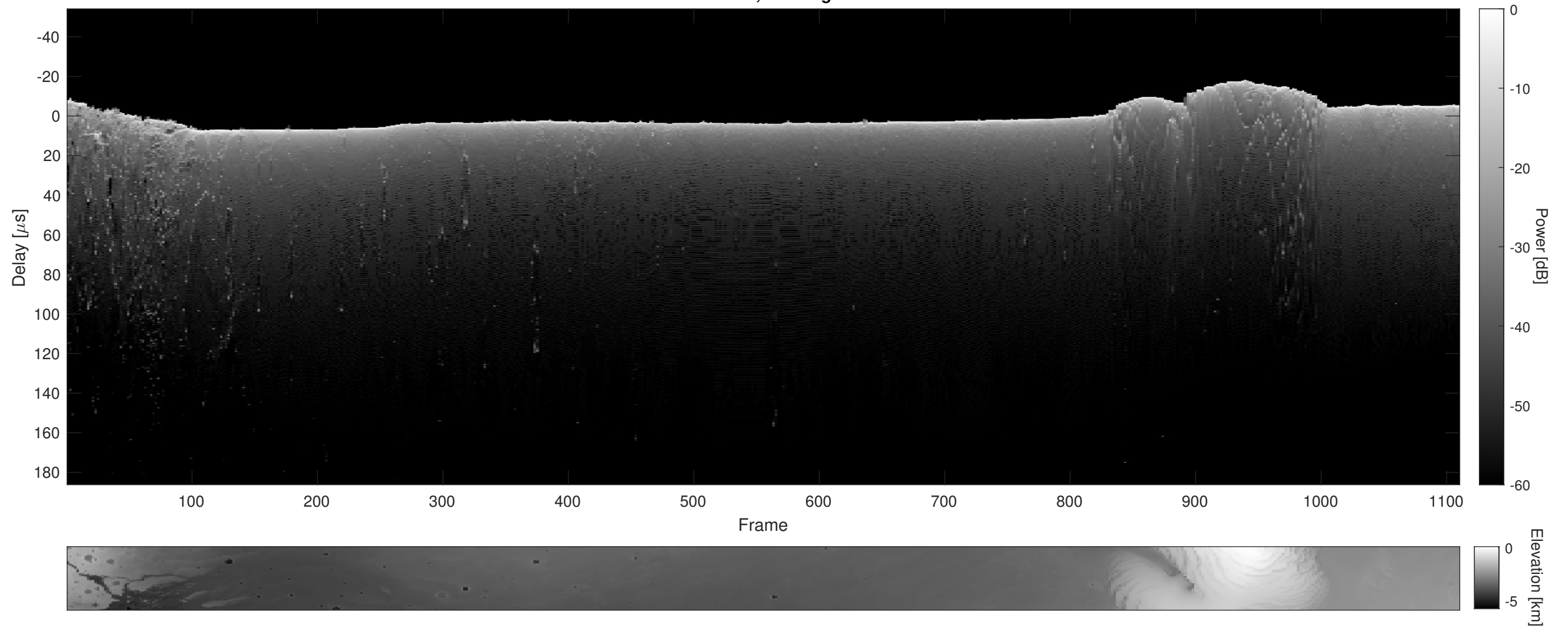
Orbit 12071, Cluttergram
