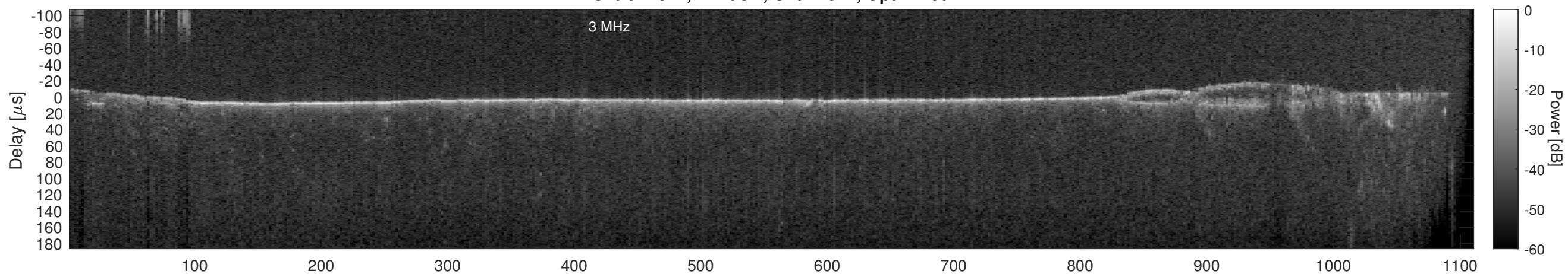
Orbit 12071, Cluttergram
