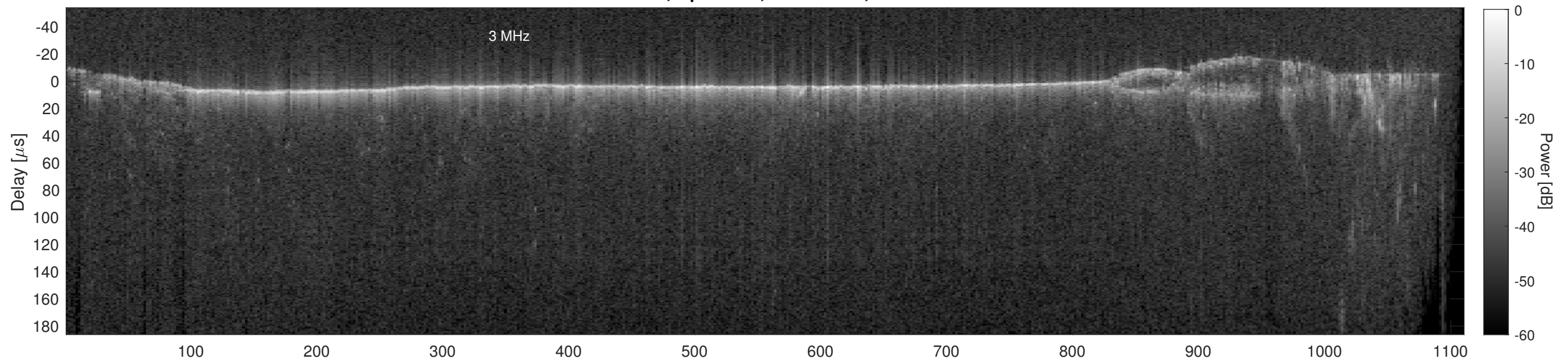
Orbit 12071, Cluttergram
