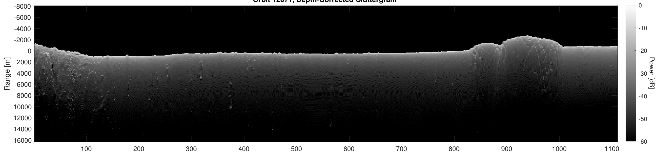
Orbit 12071, Depth-Corrected Cluttergram
