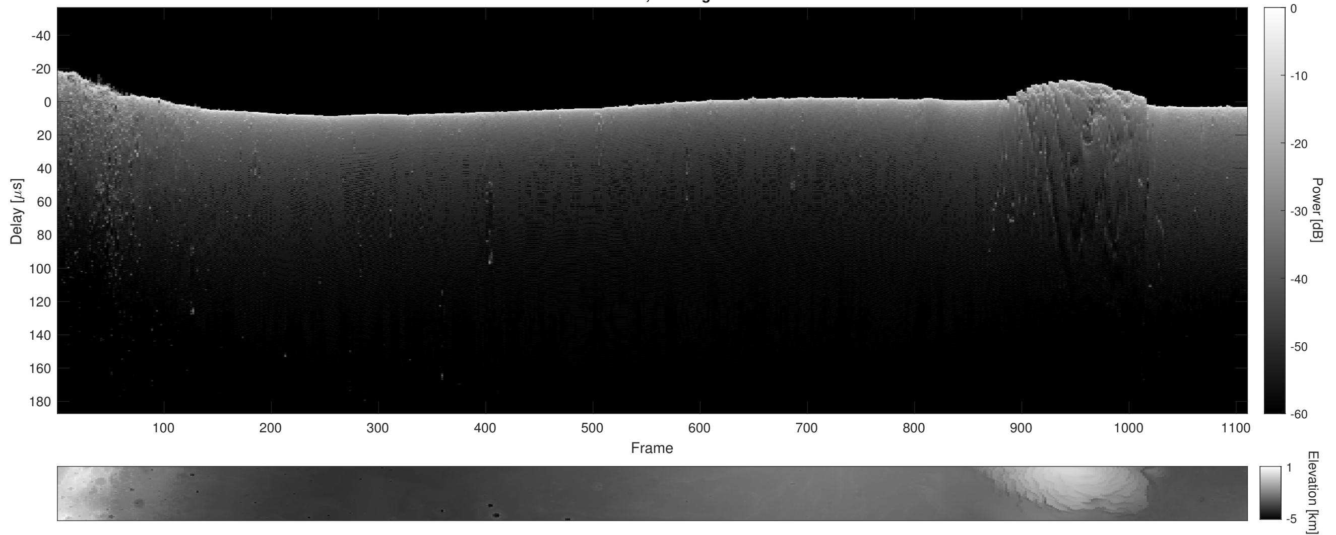
Orbit 12073, Cluttergram
