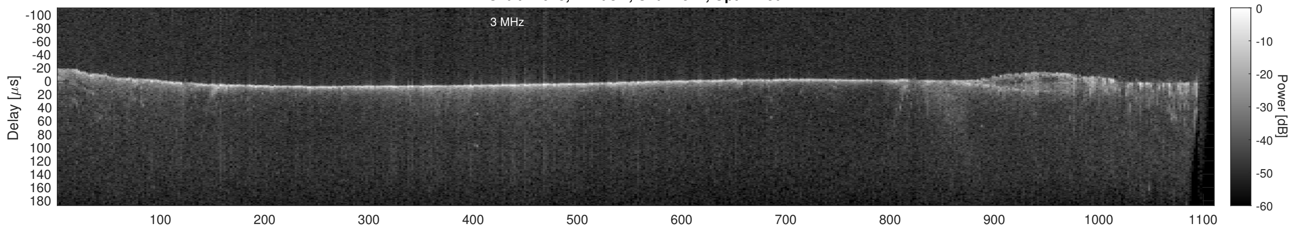
Orbit 12073, Cluttergram
