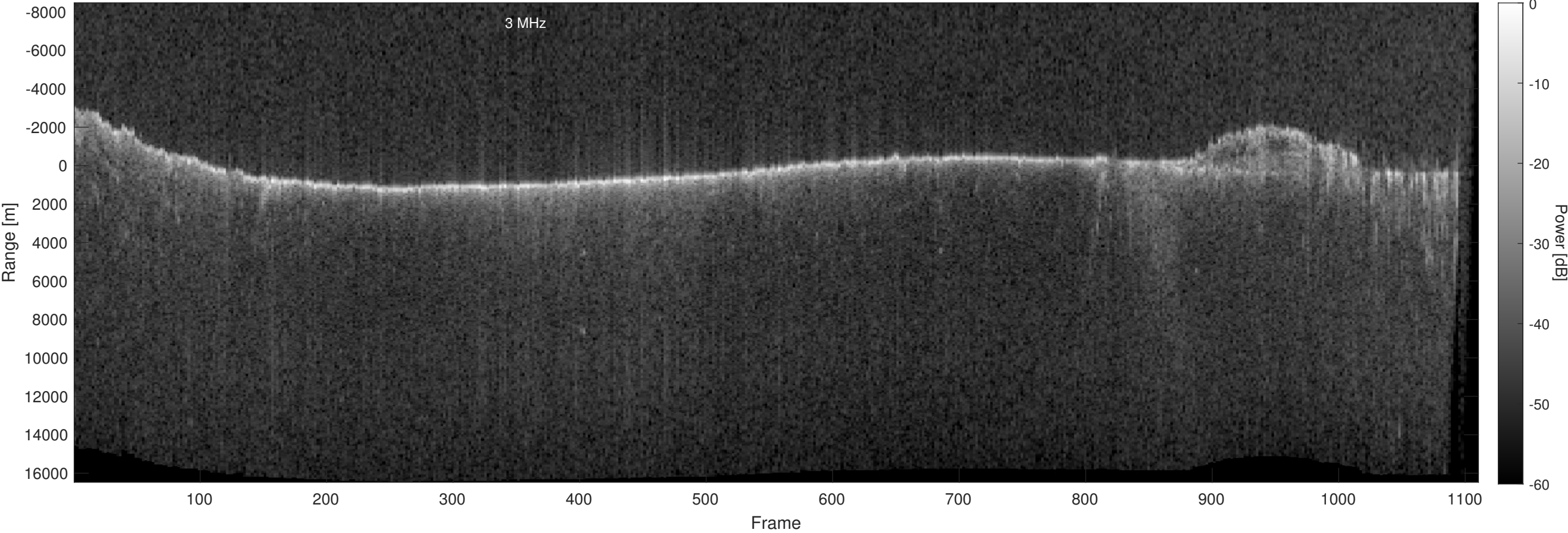
Orbit 12073, Optimized, Window, Depth-Corrected, Channel 2
