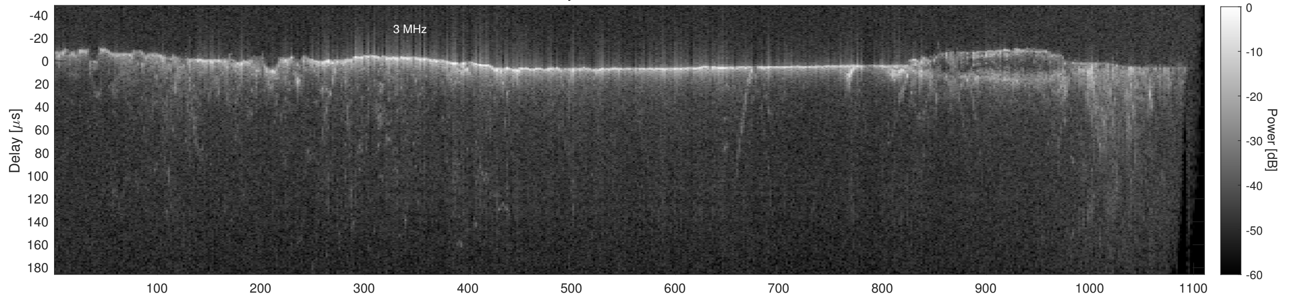
Orbit 12074, Cluttergram
