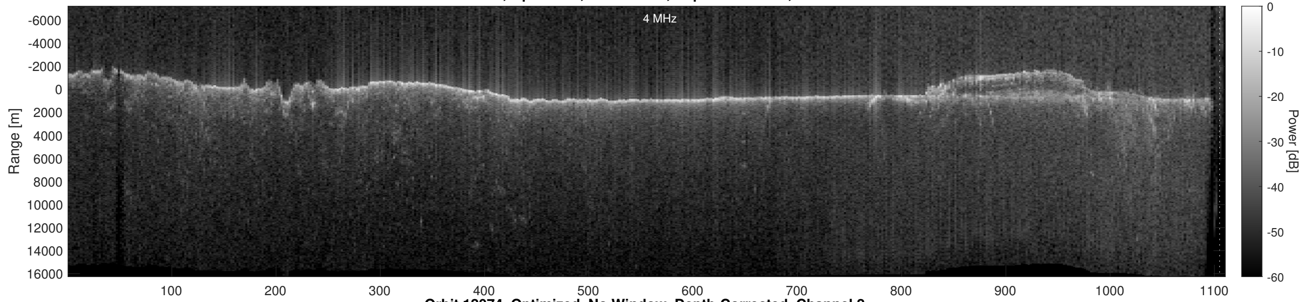
Orbit 12074, Optimized, No Window, Depth-Corrected, Channel 2
