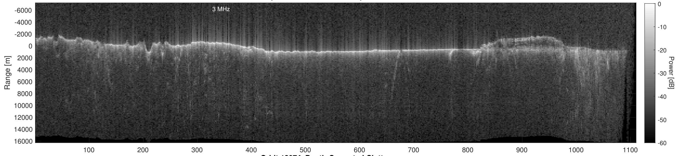
Orbit 12074, Depth-Corrected Cluttergram
