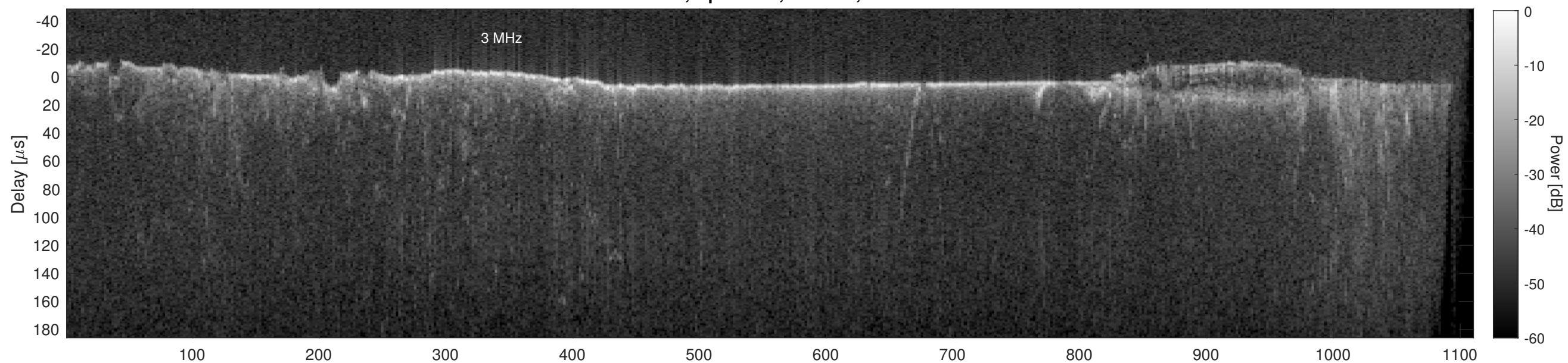
Orbit 12074, Cluttergram
