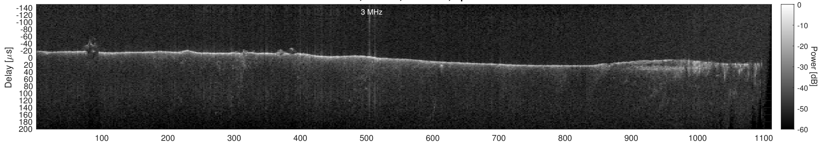
Orbit 12075, Cluttergram
