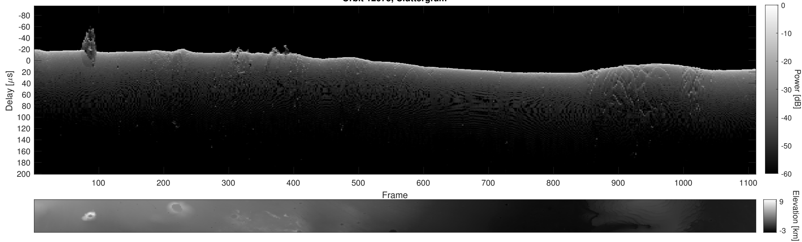
Orbit 12075, Cluttergram
