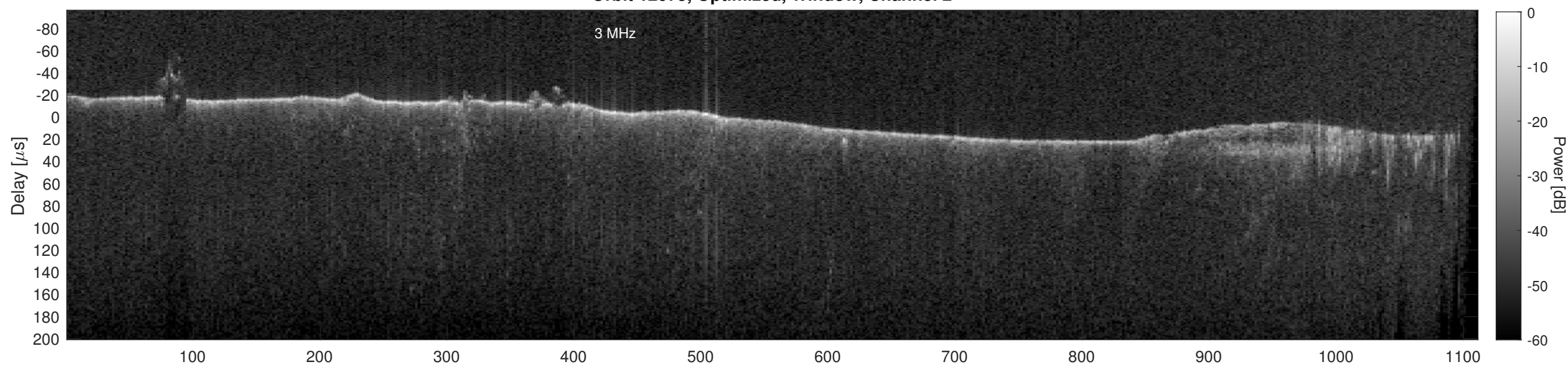
Orbit 12075, Cluttergram
