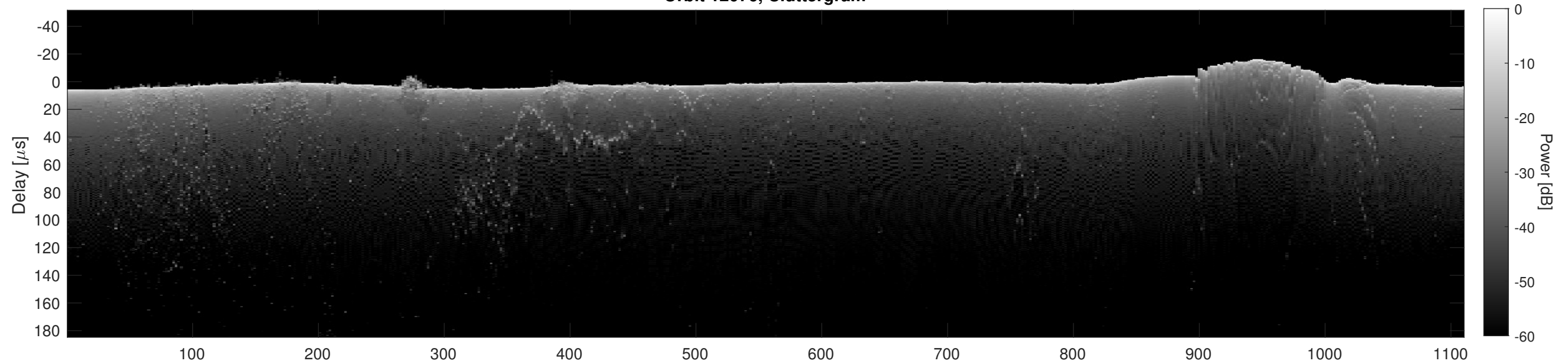
Orbit 12076, Cluttergram
