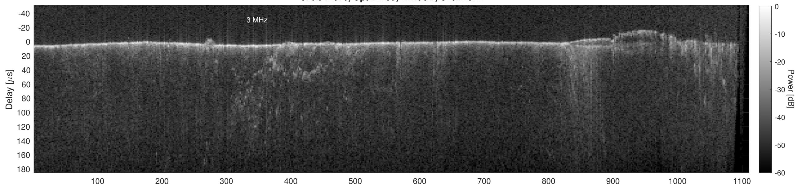
Orbit 12076, Cluttergram
