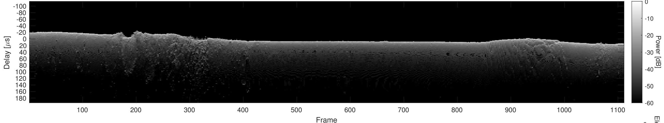
Orbit 12077, Cluttergram
